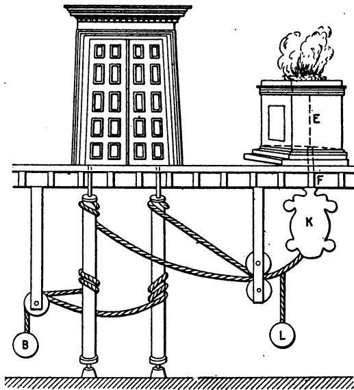
FIG. 1.—Hero's device for opening temple doors.
